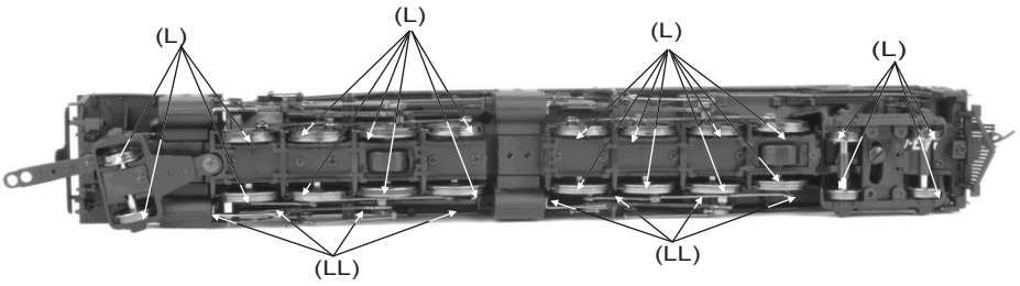
Lubricate Side Rods and Linkage(Both Sides) (LL)
