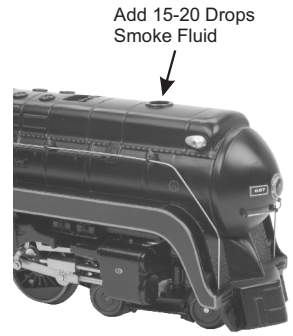
Figure 11: Adding Fluid
