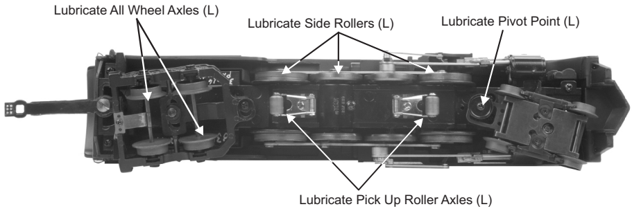
Figure 8: Lubricating the Locomotive
