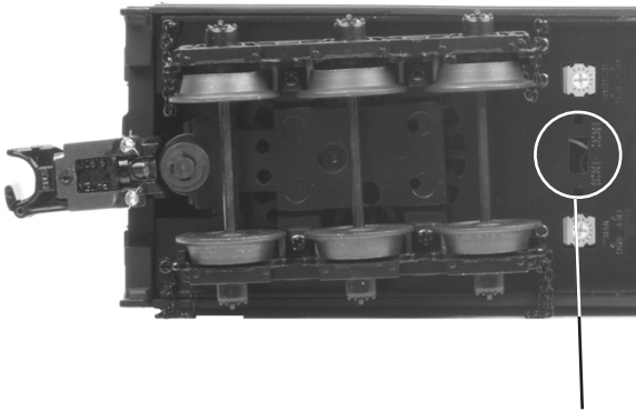
DCS/DCC Switch Location
