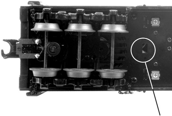
DCS/DCC Switch Location
