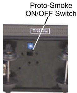
Figure 6. Smoke Switch
