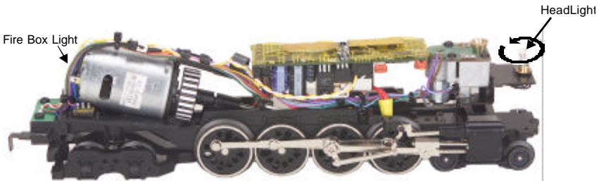
Figure 8. Replacing the Headlight and the Fire Box
