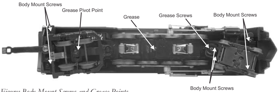
Figure: Body Mount Screws and Grease Points
