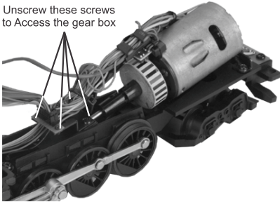
Figure: Motor Gearing Grease Plate Screws
