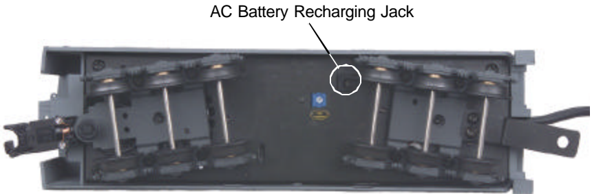
Figure 12: Battery Recharging Jack
