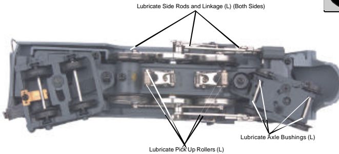
Figure 5: Lubricating The Chassis
