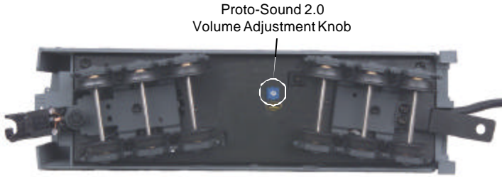
Figure 4: Manual Volume Adjustment
