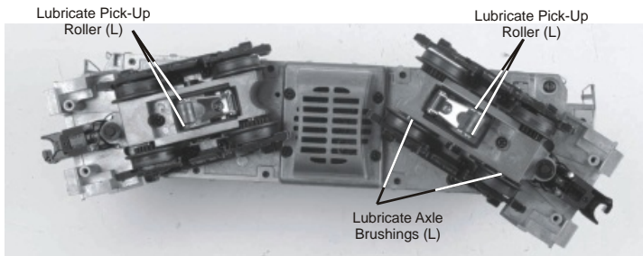
Figure 3: Lubrication Points
