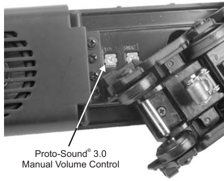
Figure 5: Manual Volume Control
