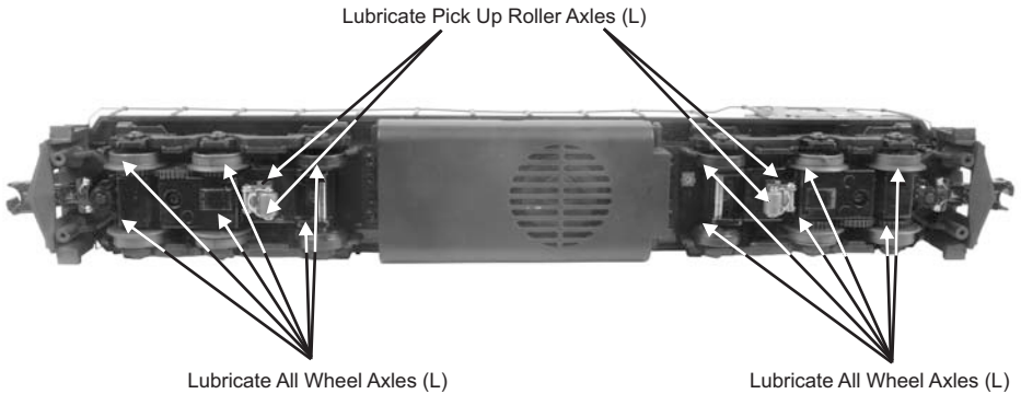
Figure 6: Lubrication Points on the Locomotive
