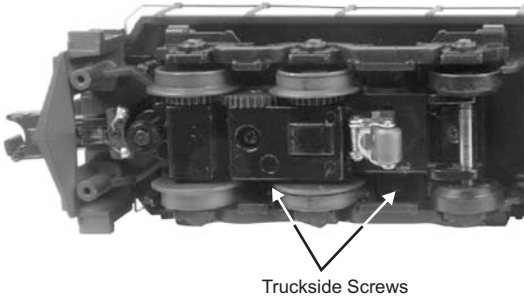
Figure 9: Truckside Screws
