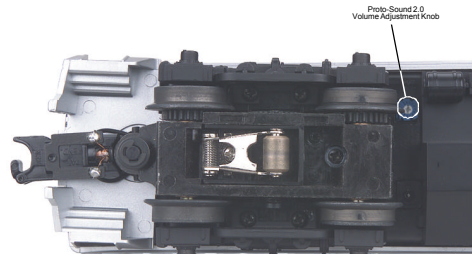
Figure 2: Manual Loco-Sound Volume Adjustment
