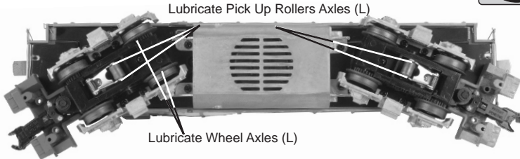
Figure 5. Lubrication Points on the Locomotive.
