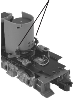
Figure 8. Replacing the Light Bulbs
