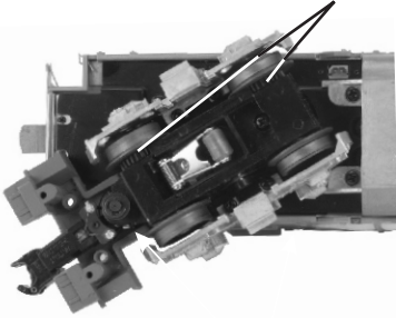
Figure 7. Greasing The Idler Gears
