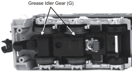
Greasing The Idler Gears
