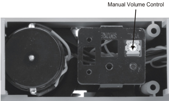
Manual Volume Control
