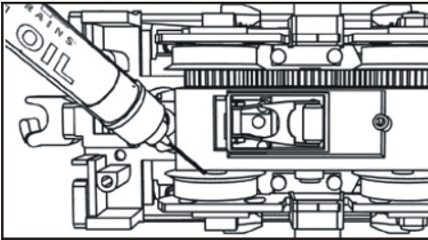
Lubricate Axles
