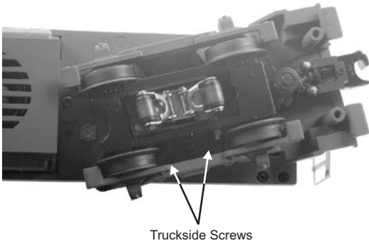
Figure 6: Truckside Screws
