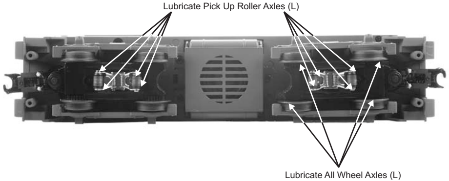
Figure 3: Lubrication Points on the Locomotive
