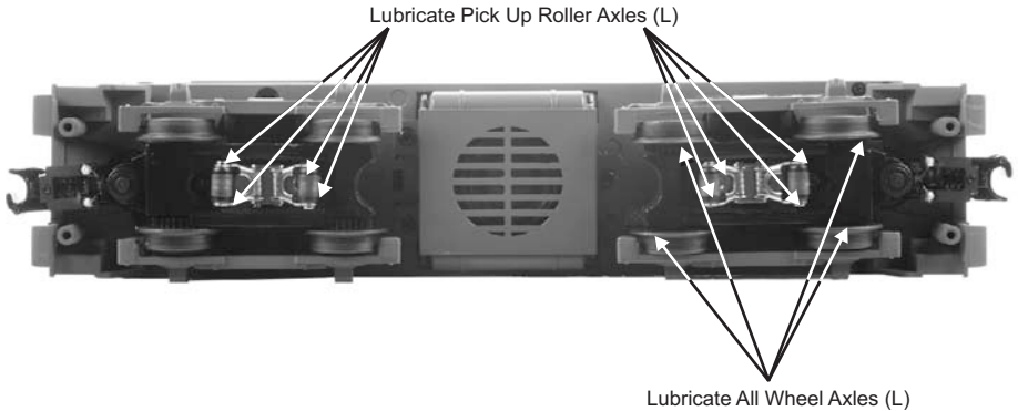
Figure 1: Lubrication Points on the Locomotive
