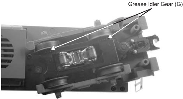
Figure 5: Greasing the Idler Gears
