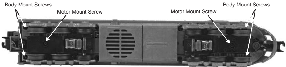
Figure 7: Body Mount Screws
