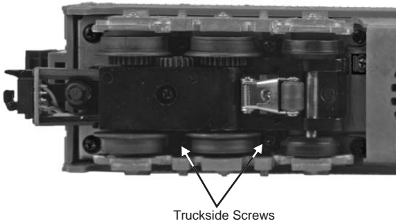
Figure 9: Truckside Screws
