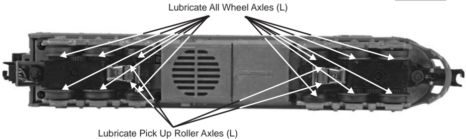
Figure 6: Lubrication Points on the Locomotive
