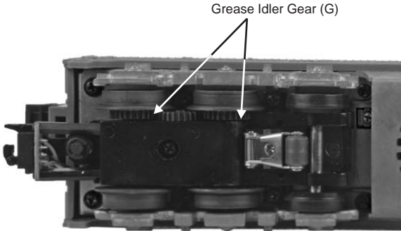
Figure 8: Greasing the Idler Gears
