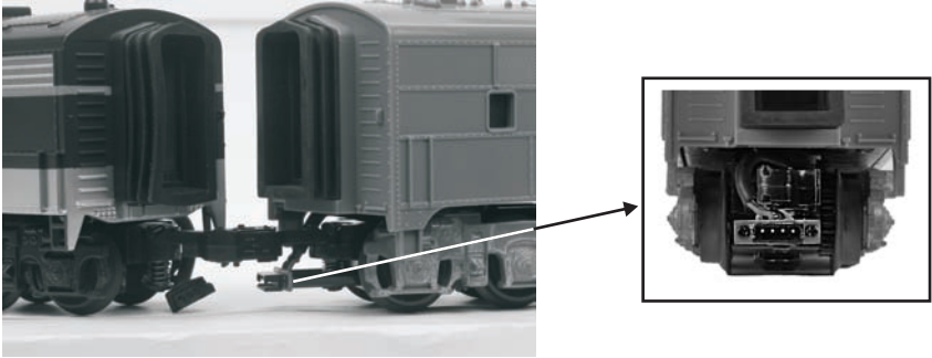
Figure 2: A Units coupled together
