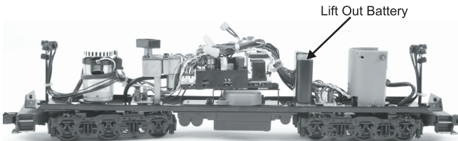
RKS FM Trainmaster Diesel Engine with PS-2
