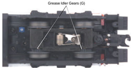
Figure 4: Greasing The Idler Gears
