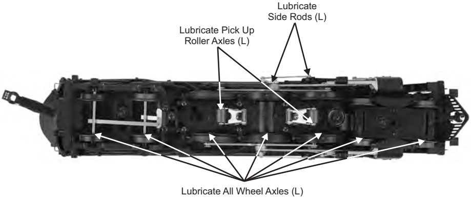
Figure: Lubricating the Locomotive
