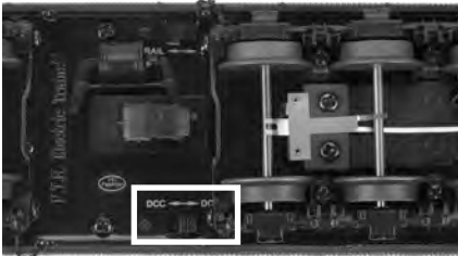
Figure: DCC-DCS Switch on Tender
