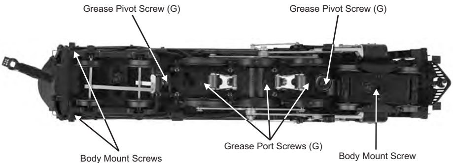
Figure: Grease Points / Body Mount Screws
