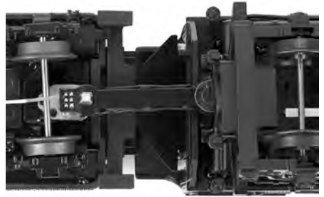
Figure: Engine and Tender
