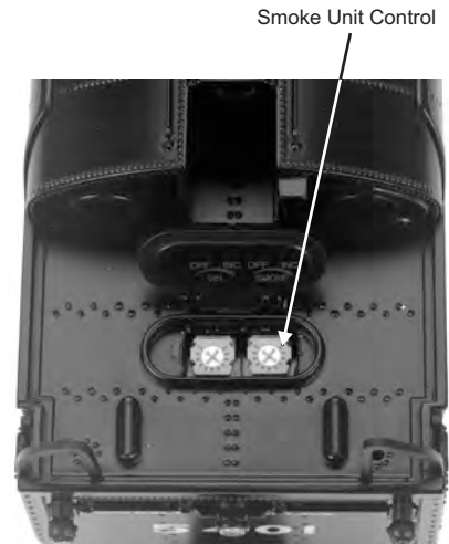
Figure: Smoke Unit Control on PT Tender
