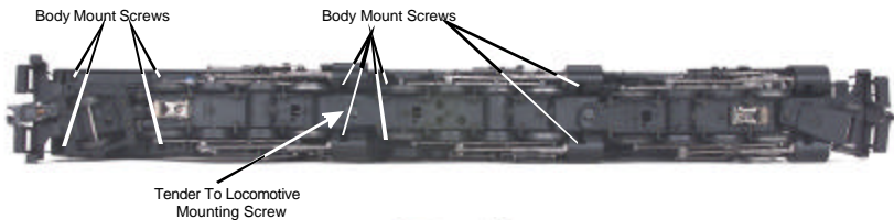
Figure 5: Removing The Body
