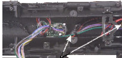
Wires for headlight & marker lights
