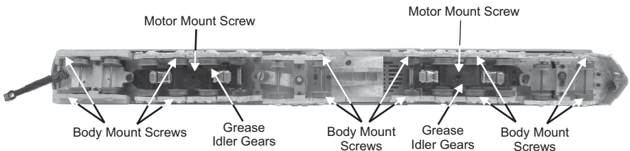
Figure: Grease Points & Body Mount Screw Locations
