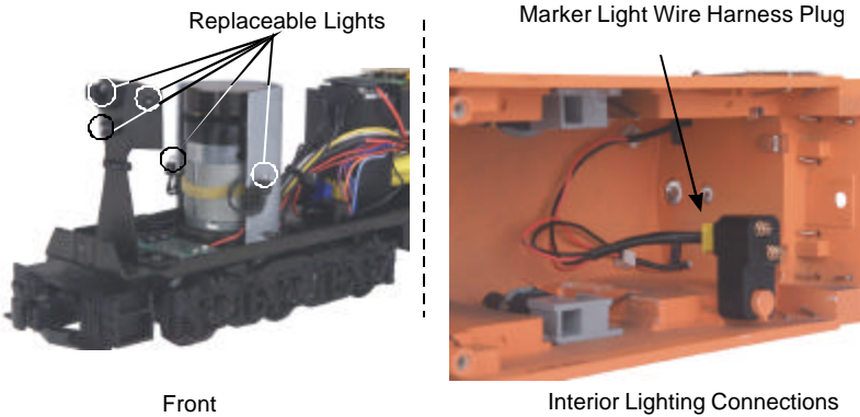
Figure 7: Removing The Replaceable Lights
