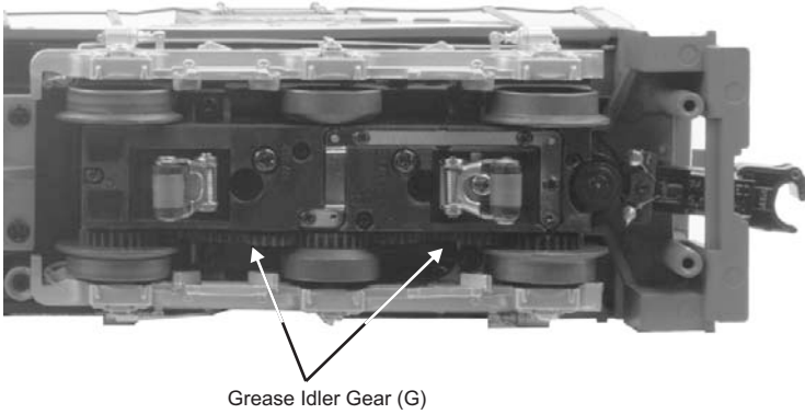
Figure 10: Greasing the Idler Gears
