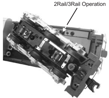
Figure 4: 3 Rail – 2 Rail Switch
