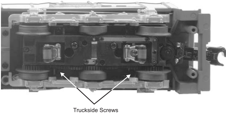
Figure 11: Truckside Screws
