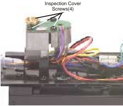
Figure 9. Inspecting the Smoke Unit Wick
