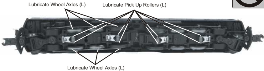
Figure 1. Lubrication Points on the Locomotive
