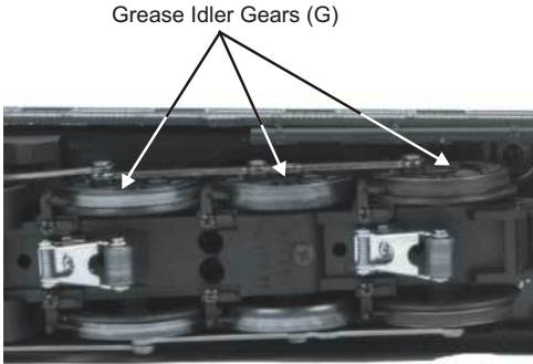
Figure 7. Greasing The Idler Gears
