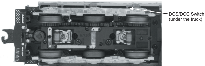
Figure 6: Changing from DCS to DCC Mode
