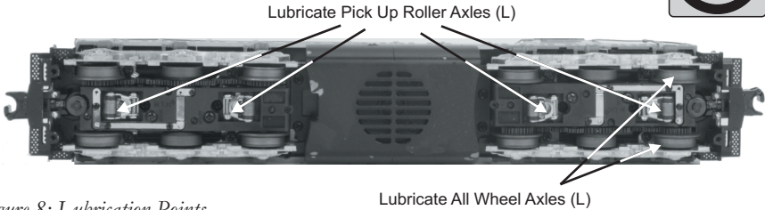
Figure 8: Lubrication Points
