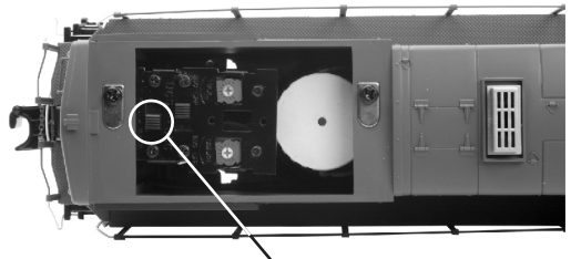
Figure 4: 2Rail/3Rail Switch & Smoke Control
