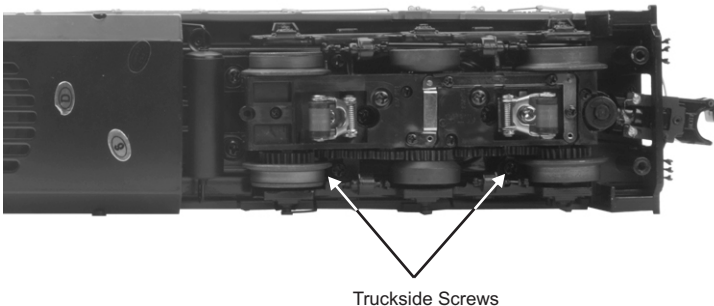
Figure 11: Truckside Screws
