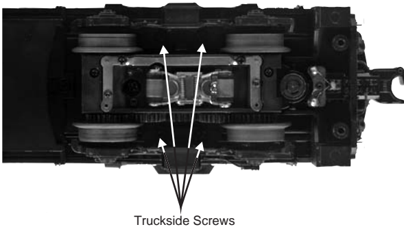
Figure 11: Truckside Screws
