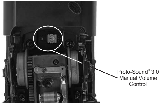
Figure 7: Manual Volume Control
