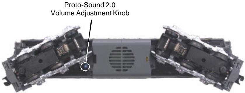
Figure 4: Manual Volume Adjustment Knob
