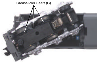
Figure 6: Greasing The Idler Gears
