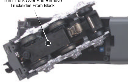
Figure 7: Removing The Truck Block To Access Truckside Screws
