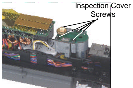
Figure 12 : Smoke Unit Inspection
