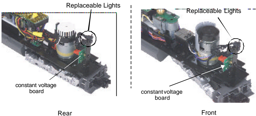
Figure 8: Removing The Replaceable Lights
