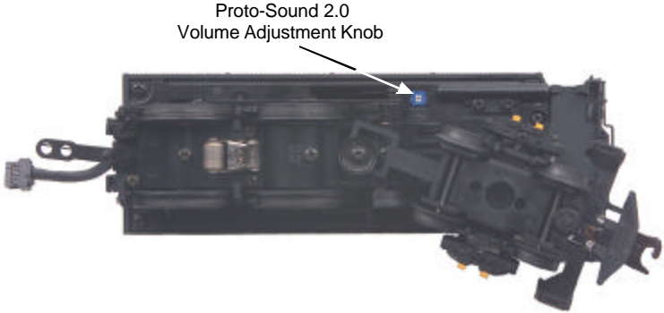
Figure 2: Manual Volume Adjustment Knob
