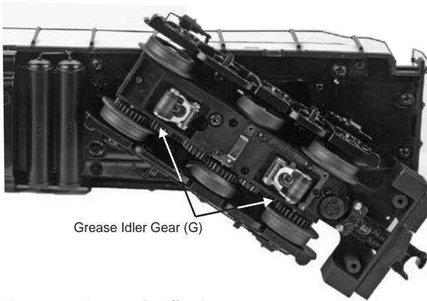
Figure 10: Greasing the Idler Gears
