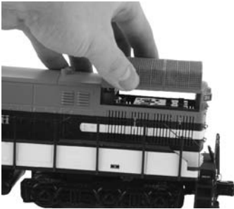
Figure 3: Accessing Smoke Unit Control
