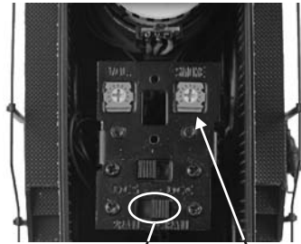
2Rail/3Rail Operation Smoke Unit Control Figure 4: Smoke Unit Control + 2Rail/3Rail Switch
