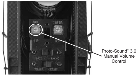
Figure 7: Manual Volume Control
