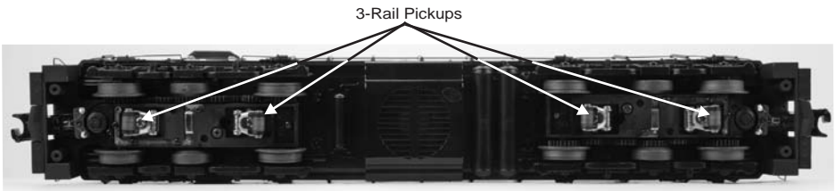
Figure 5: 2-Rail/ 3-Rail Operation
