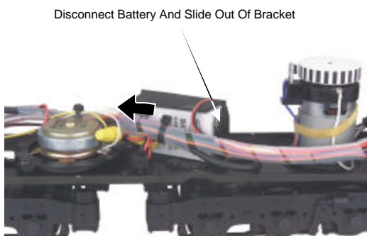
Figure 7: Removing The Battery
