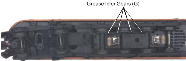
Figure 4: Greasing The Idler Gears
