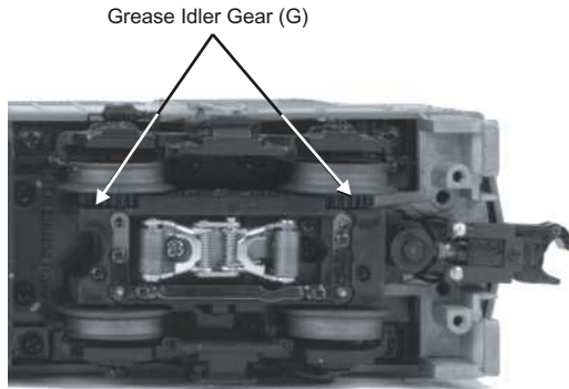
Figure 11. Greasing The Idler Gears
