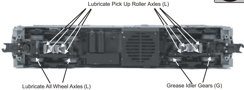
Figure 8. Lubrication points on the Locomotive
