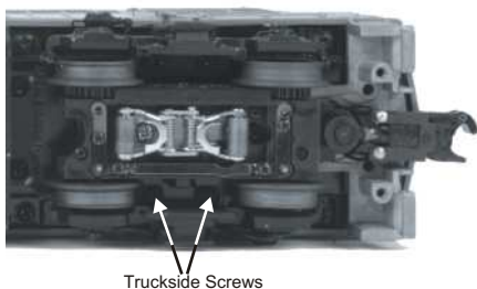
Figure 12. Truckside Screws
