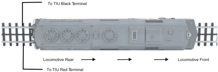
Figure 5: Proper 2-Rail polarity wiring and locomotive orientation
