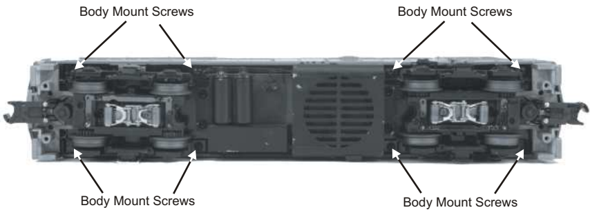
Figure 13. Body Mount Screw Locations
