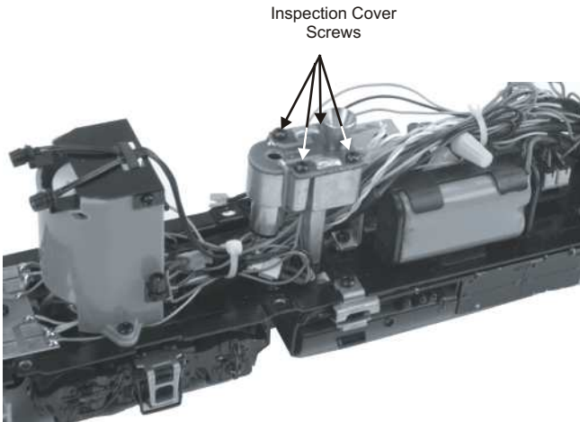
Figure 17. Inspecting the Smoke Unit Wick
