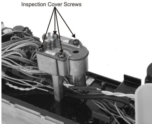
Inspecting the Smoke Unit Wick
