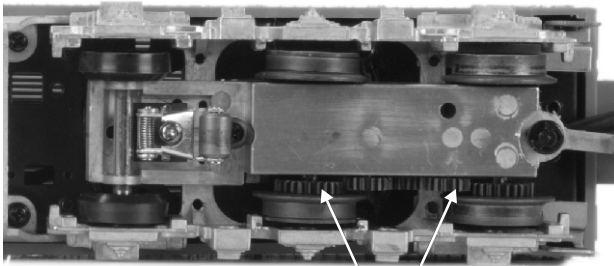
Grease Idler Gear (G)
