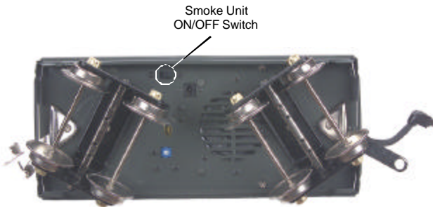
Figure 5: Smoke Unit Switch Location
