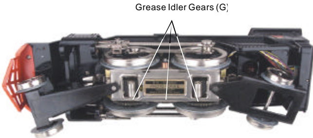
Figure 10: Greasing the Idler Gears
