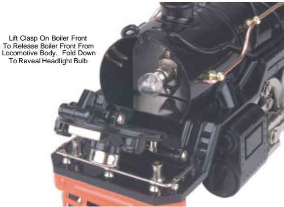
Figure 11: Replaceable light bulb locations
