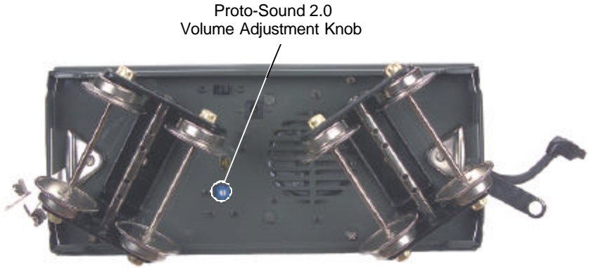
Figure 6: Proto-Sound Manual Volume Adjustment
