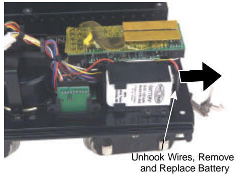
Figure 13: Removing the battery
