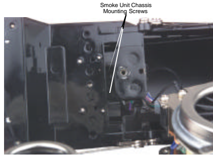
Figure 15: Removing The Smoke Unit Assembly
