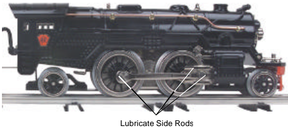
Figure 2: Lubricating Side Rods
