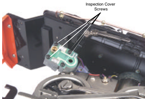
Figure 16: Inspecting The Smoke Unit Wick
