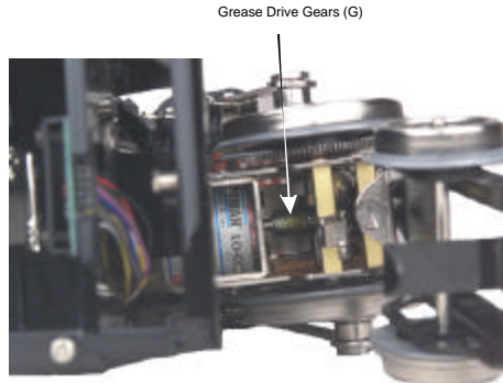
Figure 9: Greasing the gears
