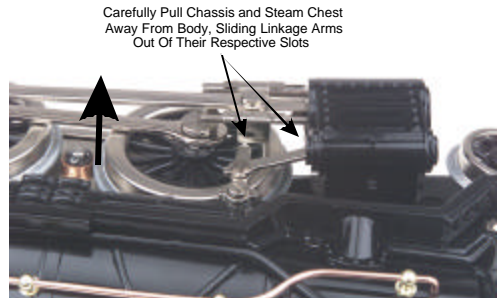
Figure 8: Removing The Leading Truck
